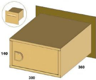
Model FR60MBRR
